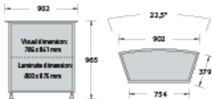
Q 400.31 Basic set, silver-grey RAL 9006
